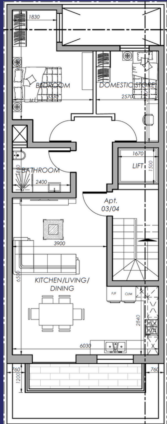
PROPOSED LEVELS 3&4
