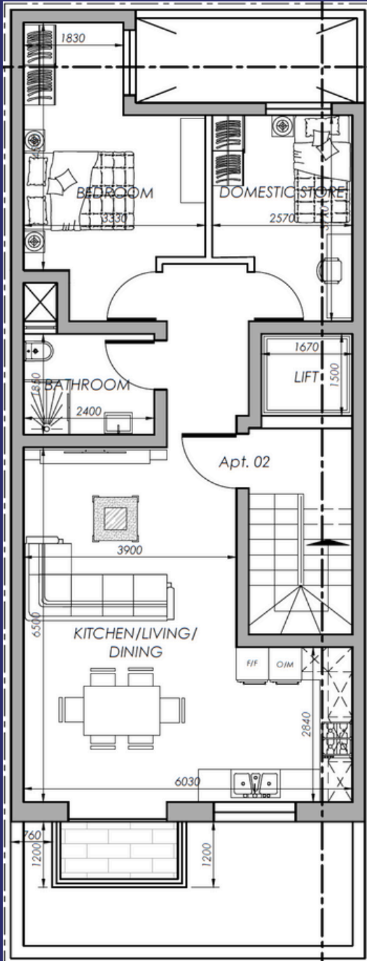
PROPOSED LEVEL 2
